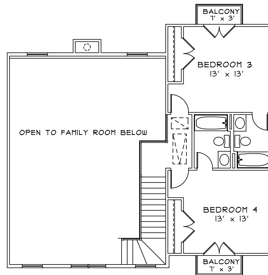
2ND FLOOR
