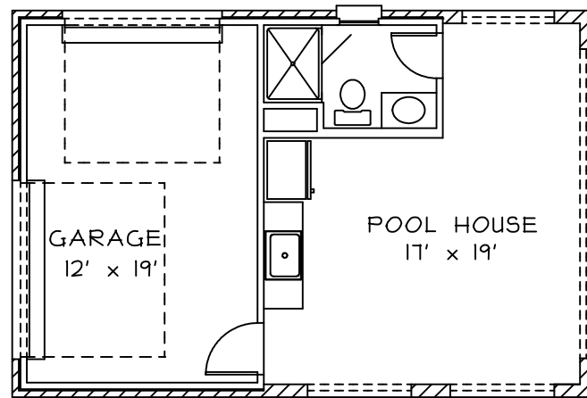
GARAGE/POOL HOUSE
