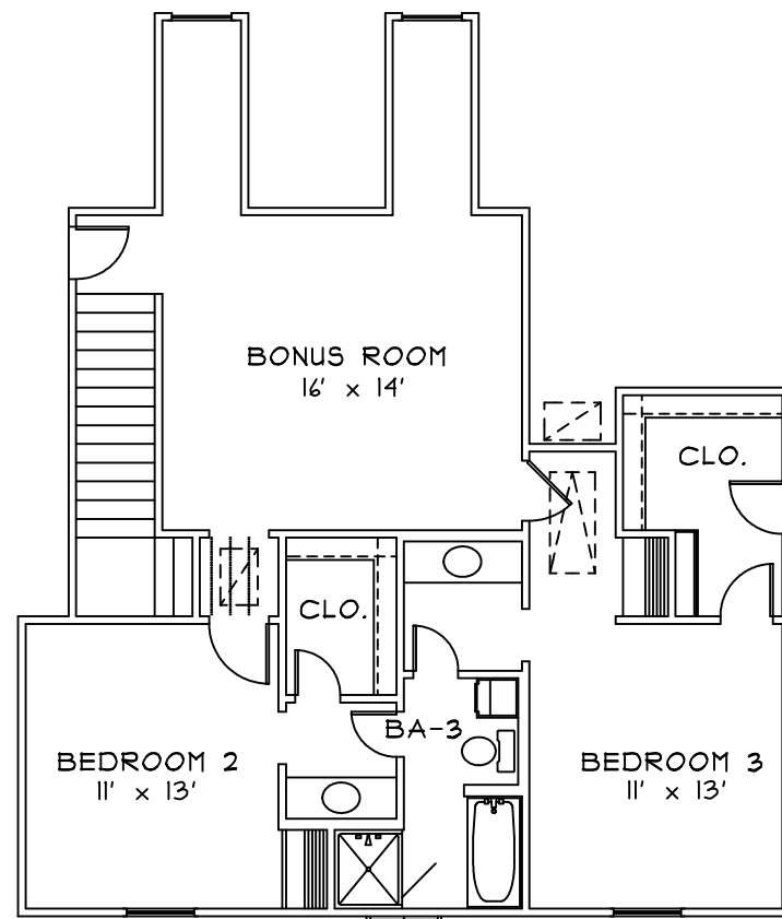
2ND FLOOR
