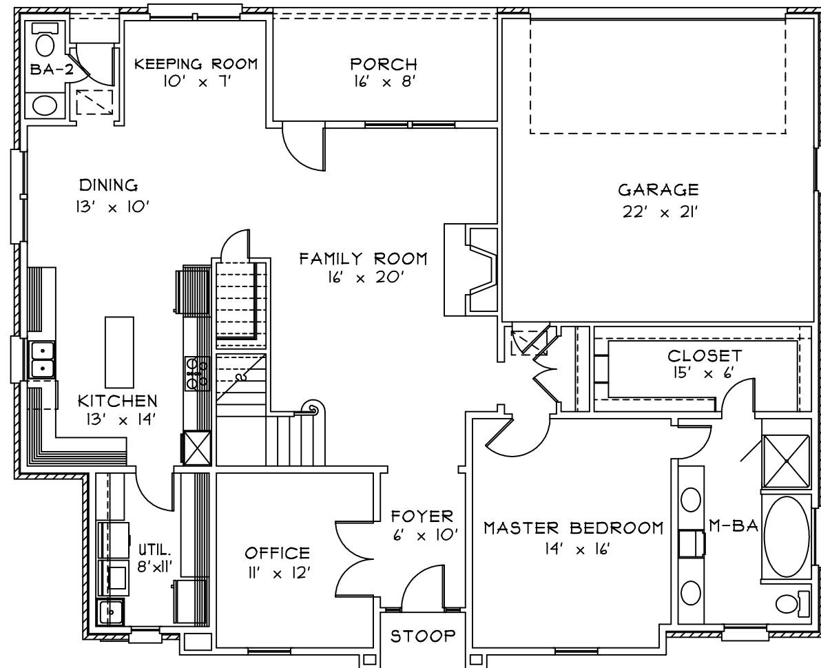
1ST FLOOR
