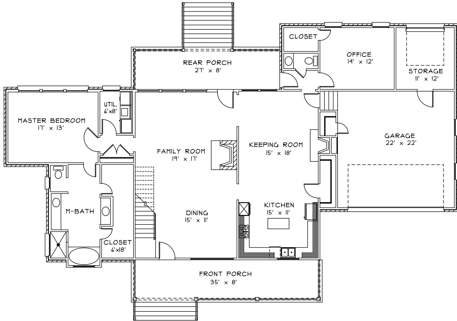
1ST FLOOR
