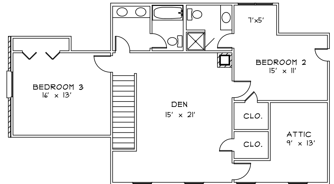
2ND FLOOR
