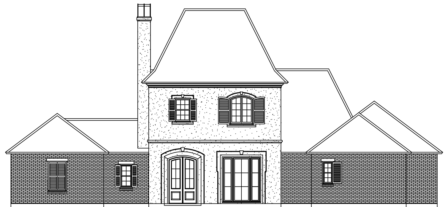
FRONT ELEVATION
